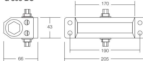
Diagram G 805 BC
