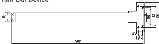
Diagram RIM Exit Device
