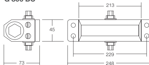
Diagram G 806 BC
