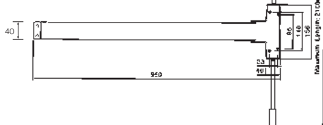
Diagram Vertical Exit Device
